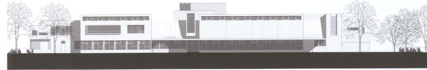
North elevation
